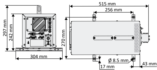
Tank Unit
