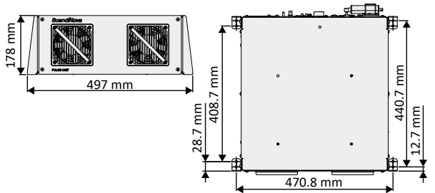
Pulse Unit
