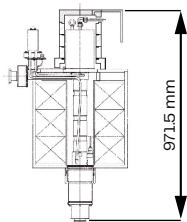
Klystron and Solenoid
